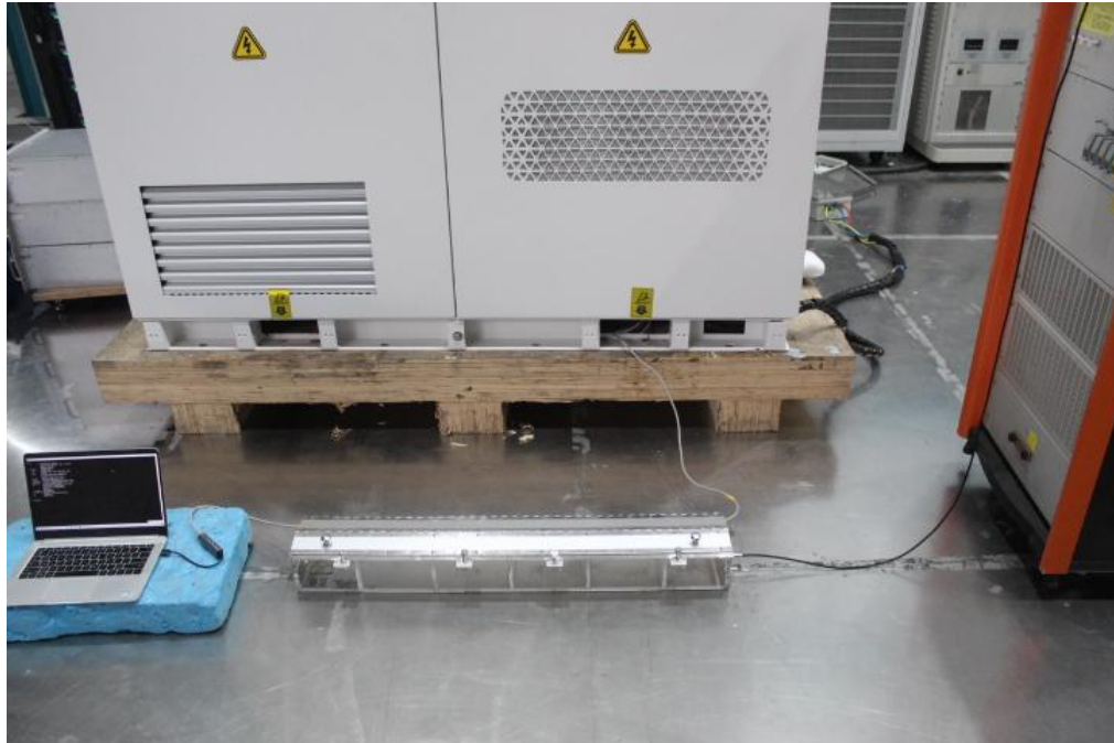
(Signal port)
