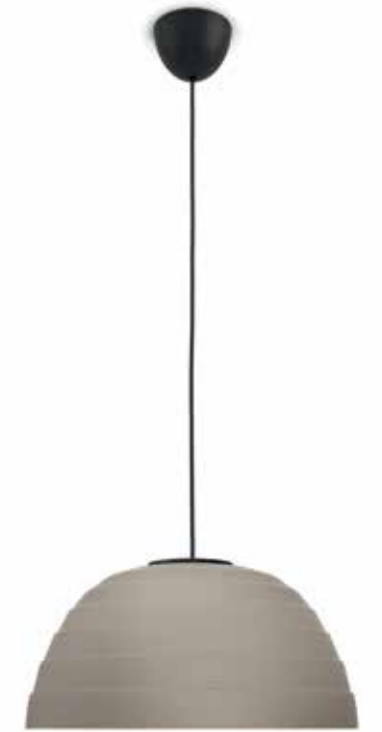
Var 40895/87/16 1 1500 → 350 / 350 LED - 1x 4,5W incl. - 430 lm ☐ - IP20 metal
