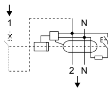
Wiring diagram
