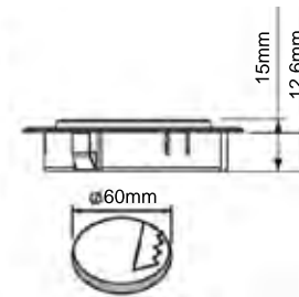
Cut-out size: Ø60mm
