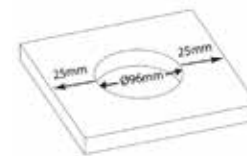
Cut-out Ø96mm
