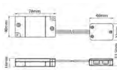
RGB & DuoFlex - 4 ports
