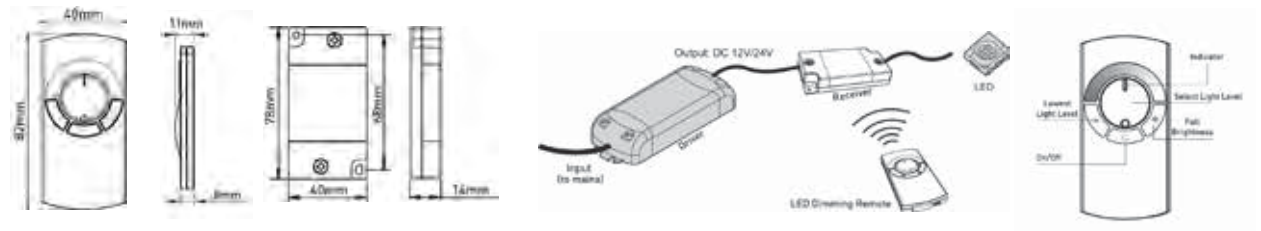
LED Dimming Remote Control
