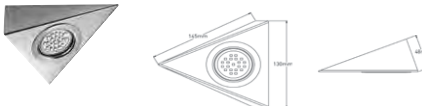
LED Triangle Light
