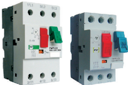
Motor protection circuit breakers FMP2 (0.63-80A)
