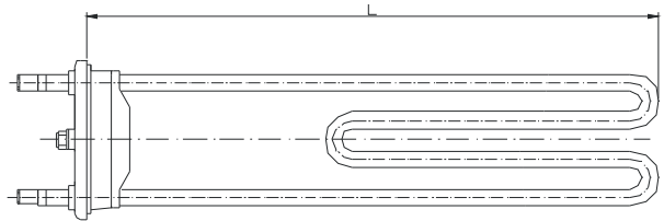
Heating element for washing machine with plastic drum - seal height approx. 18 mm
