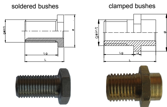
Tubular heating elements
