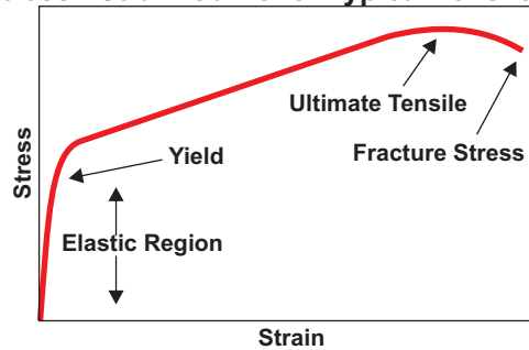
Stress - Strain Curve for Typical Tensile Test
